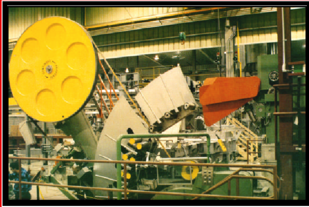
12 t/h Aluminum Caster
